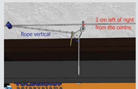
Placing of the pulley/wire clip and knotting of the rope
