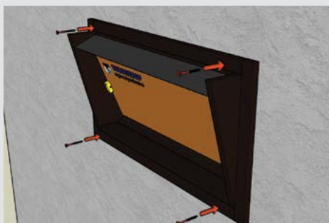
Screw inlet in upper and lower flange
